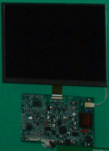
PVI80X51 8" M1023A, 1700x1050, NTSC/PAL, CCFL, 330cd/m²
